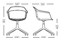
4 Spoke base with pads chair Base 4 brazos tapones - Giratoria
